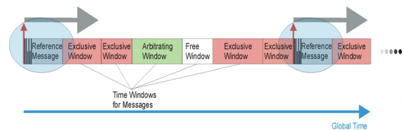
Figure 4 - Exclusive time windows and arbitrating time windows of a TTCAN basic cycle.
