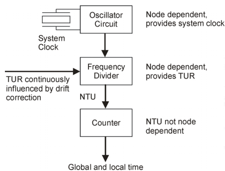
Figure 9 - Generation of NTU and the influence of TUR
