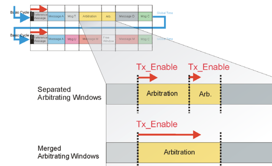
Figure 7 - Merged arbitrating windows
