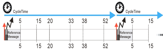
Figure 8 - TTCAN's cycle time and the time marks
