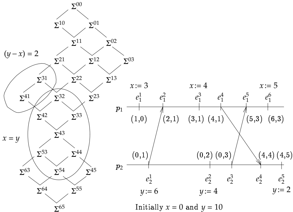
Figure 16. Global States Satisfying Predicates (x = y) and (y - x) = 2
