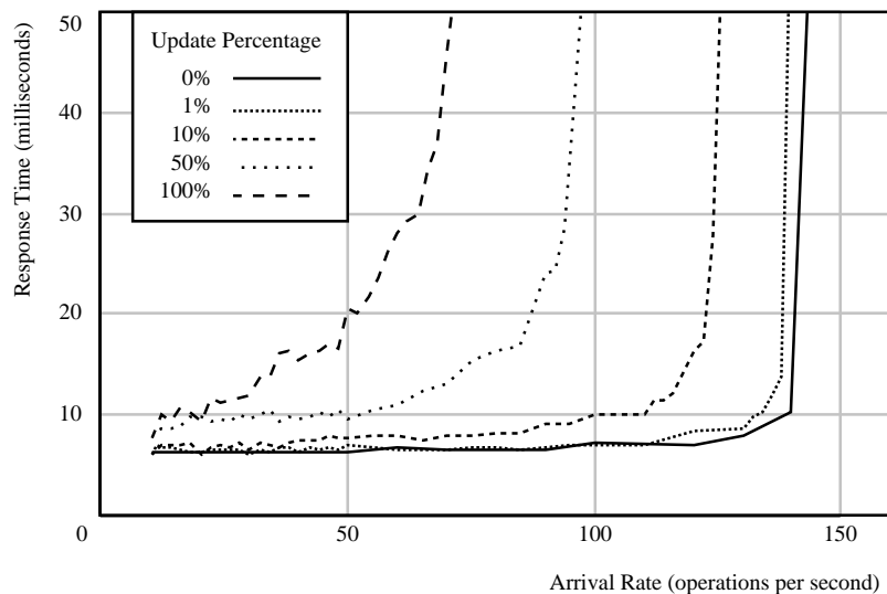
Figure 3-2: Capacity of a Single Replica. This figure shows the average response time as a function of operation arrival rate for selected operation mixes.
