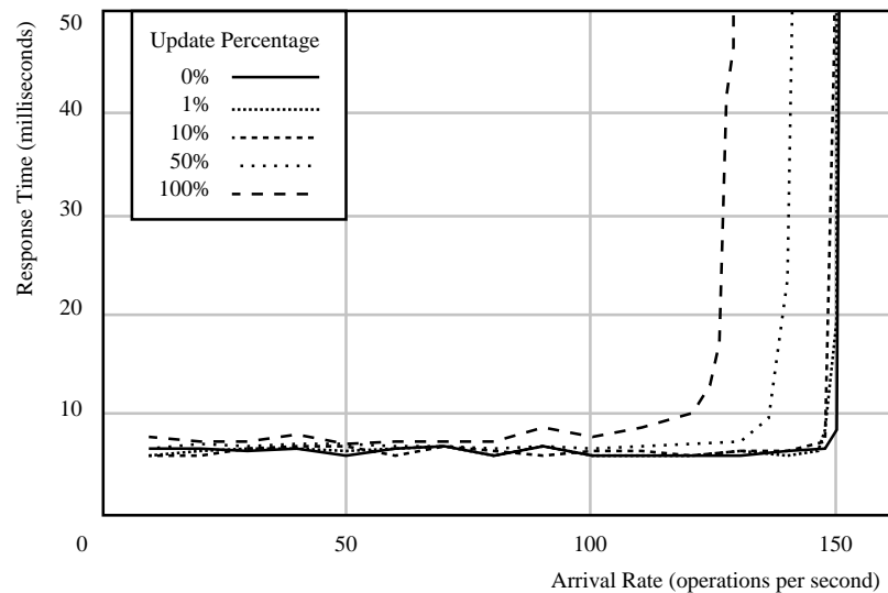
Figure 3-3: Capacity of the Unreplicated System.
