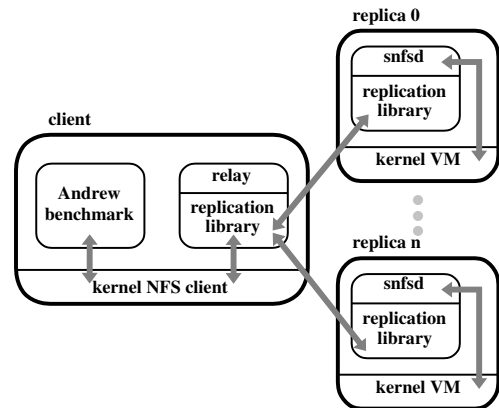
Figure 2: Replicated File System Architecture.
