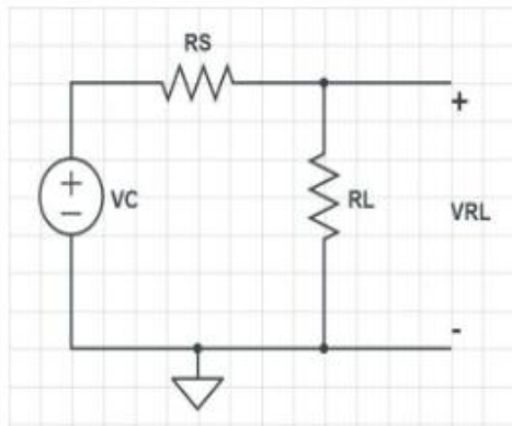
Figure 6: Circuit Simplified
